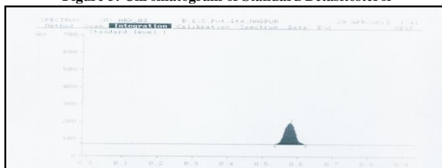
Figure 6: Overlain spectrum of betasitosterol, standard and oil formulation
