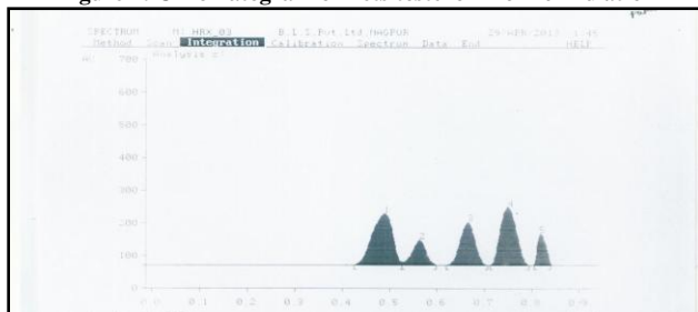
Figure 5: Chromatogram of Standard Betsitosterol
