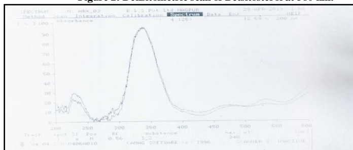
Figure 2: Densitometric scan of Betsitosterol at 560 nm.
