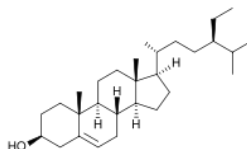
Figure 1: Chemical structure of Betsitosterol
