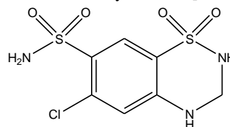
Fig.1. Chemical Structure of Hydrochlorothiazide
