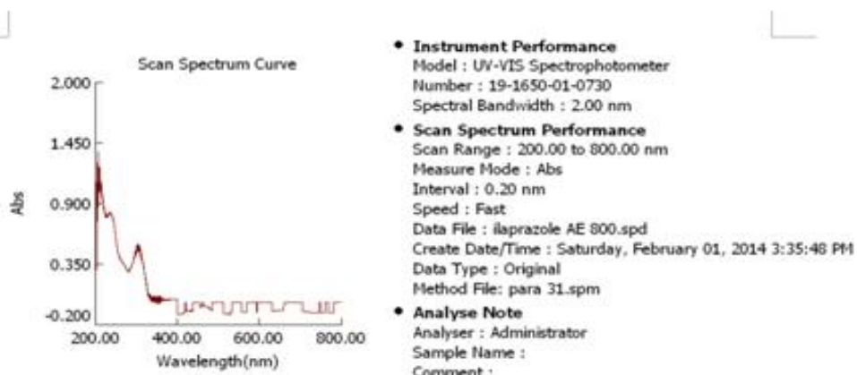
Fig no: 1 UV spectrum of Ilaprazole
