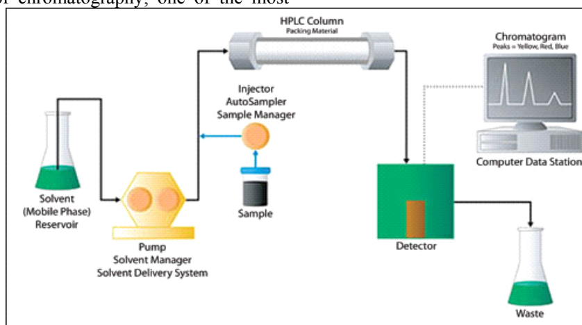
Figure 1: Block diagram of HPLC instrumentation
