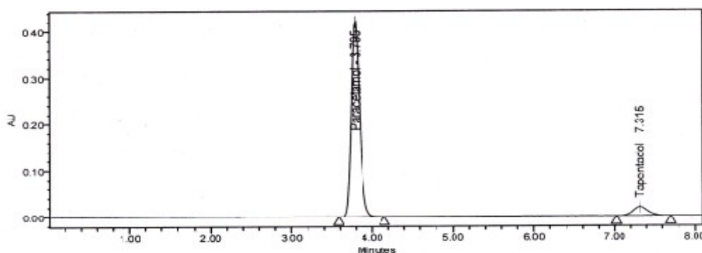
Figure 6: Chromatogram obtained by using Phosphate buffer pH 3.0
